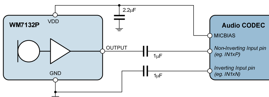
Figure 3 WM7132P Silicon Microphone Pseudo-differential Connection
